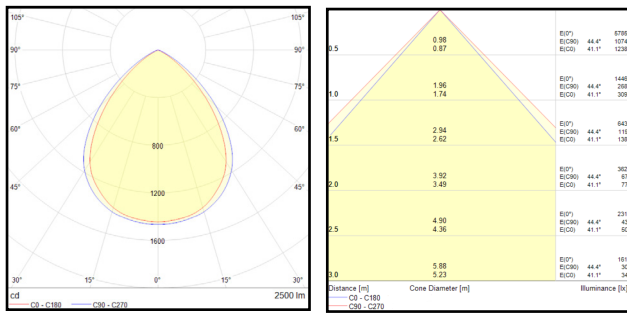
LED Downlight Spectre SR IP54 25W 5700K
