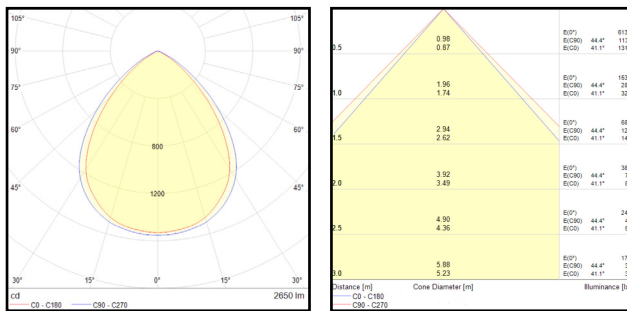
LED Downlight Spectre SR IP54 25W 5700K
