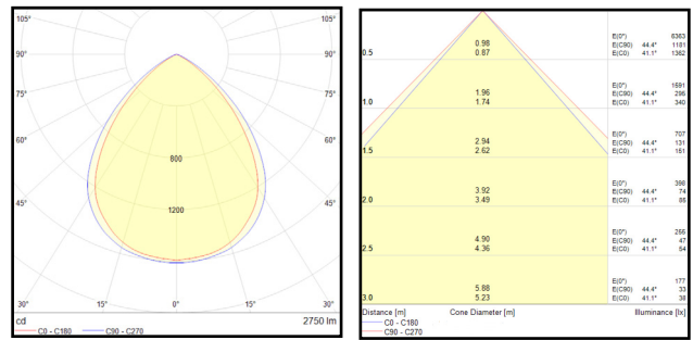
LED Downlight Spectre SR IP54 25W 4000K
